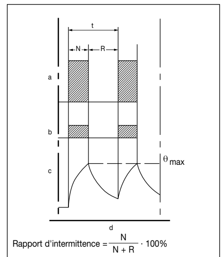
Figure 3D - Régime S3
